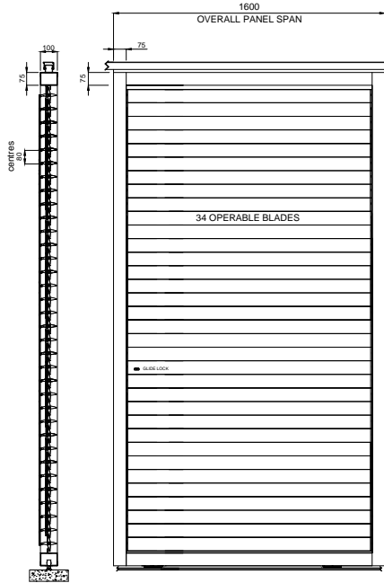
1600mm SINGLE SPAN HEAVY DUTY FRAMED BOTTOM ROLLING PANEL 75x100x3mm horizontal rails & vertical stiles. 90mm Operable Louvres .
