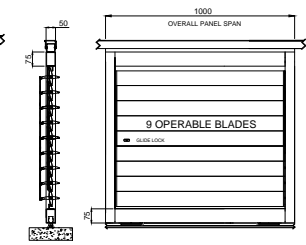
1000mm SINGLE SPAN SHUTTER PANEL 90mm Louvres - bottom rolling. 75x50x3mm horizontal rails, 50x50x3mm vertical stiles
