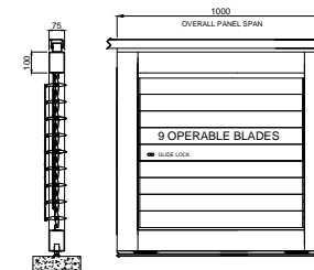
1000mm SINGLE SPAN SHUTTER PANEL 90mm Louvres - bottom rolling .
