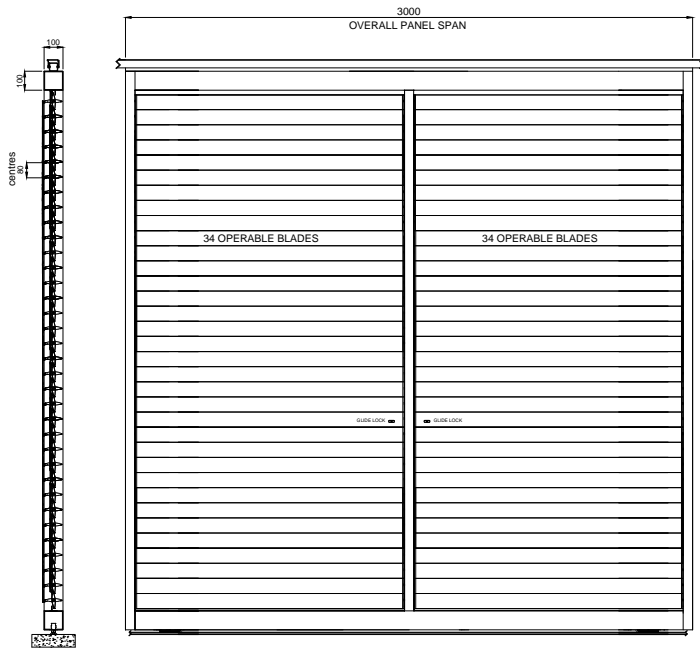
3000mm DOUBLE SPAN HEAVY DUTY FRAMED BOTTOM ROLLING PANEL 100x100x3mm horizontal rails 100x50x3mm vertical stiles & central mullion 90mm Operable Louvres.
