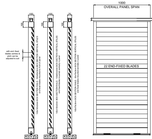
1000mm SINGLE SPAN HEAVY-DUTY FRAMED - END FIXED SHUTTER PANEL 90mm Louvres - bottom rolling.
